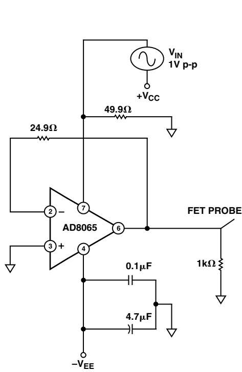
Test Circuit 7. Positive PSRR
