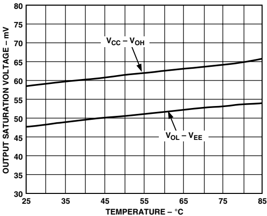
TPC 35. Output Saturation Voltage vs. Temperature
