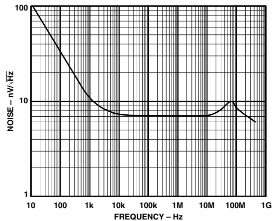
TPC 18. Voltage Noise
